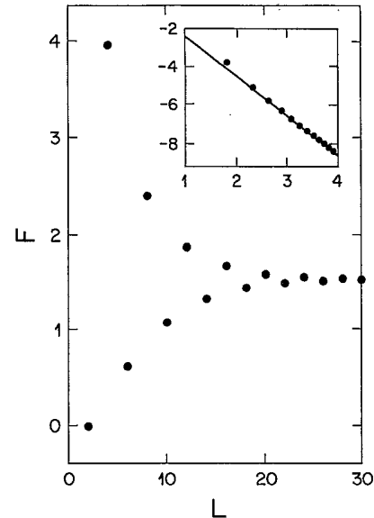
FIG. 3. Finite frequency spectral weight F = -(\pi/2L)\langle T \rangle - \pi D as a function of system size for U=4 . Inset: Finite-size corrections to the total spectral weight displayed on a log-log plot for U=10 , showing L^{-2} behavior.
