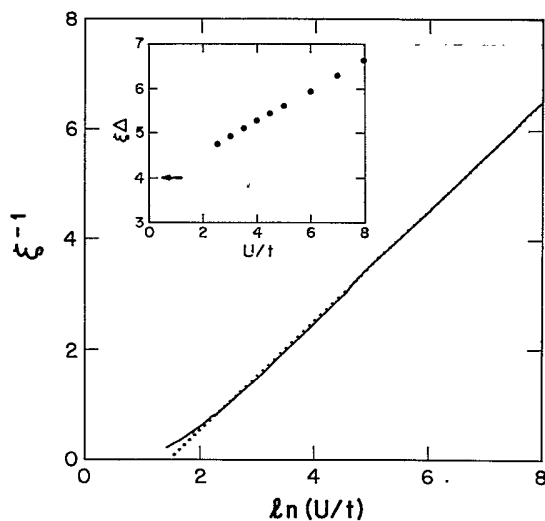
FIG. 2. The inverse of the localization length, \xi , vs \ln(U/t) . The analytic result \xi^{-1} = \ln(U/t) - 1.48 for U \gg t is shown as a dashed line. Note that \xi \rightarrow \infty as U \rightarrow 0 . Inset: \xi\Delta vs U/t , where \Delta is the Lieb-Wu charge gap. \xi\Delta appears to approach the mean-field result \xi\Delta/t = 4 (indicated by an arrow) as U \rightarrow 0 .
