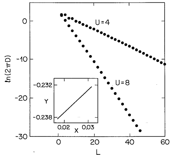
FIG. 1. \ln|2\pi D| as a function of system size for U=4 (upper curve) and U=8 (lower curve). \pi D is the dc spectral weight in units where e = \hbar = 1 . Inset: A plot of y = \ln[D(L)/D(40)]/(L-40) vs x = \ln[L/40]/(L-40) for L=42-100 and U=4 , displaying the asymptotic form y = -\xi^{-1} + \eta x . Here x = 4.06 and \eta = 0.45 .
