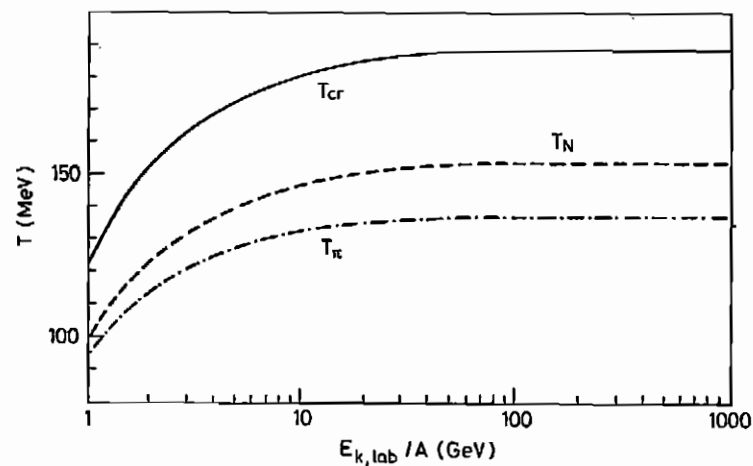
Figure 4 : Mean temperatures for nucleons and pions together with the critical temperature belonging to the point where the "cooling curves" start off the critical curve (see Fig. 2a). The mean temperatures are obtained by integrating along the cooling curves. Note that T_N is always greater than T_\pi .
