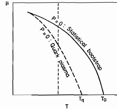
Figure 1a : The critical curves ( P = 0 ) of the two models in the T - \mu plane (qualitatively). The region below the full line is described by the statistical bootstrap model, the region above the broken line by the quark-gluon plasma. The critical curves can be made to coincide.
