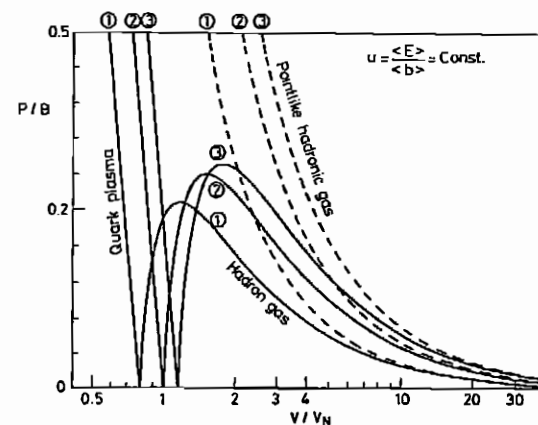
Figure 3 : P - V diagram of "cooling curves" belonging to different kinetic lab. energies per nucleon: (1) 1.8 GeV; (2) 3.965 GeV; (3) 5.914 GeV. In the history of a collision the system comes down the quark lines and jumps somewhere over to the hadron curves (Maxwell). Broken lines show the diverging pressure of pointlike bootstrap hadrons.
