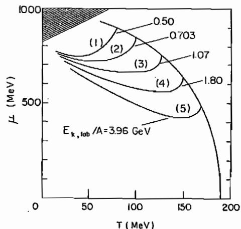
Figure 2a : The critical curve of hadron matter (bootstrap) together with some "cooling curves" in the T - \mu plane. While the system cools down along these lines it emits particles; when all particles have become free, it comes to rest on some point on these curves ("freeze out"). In the shaded region our approach may be invalid.
