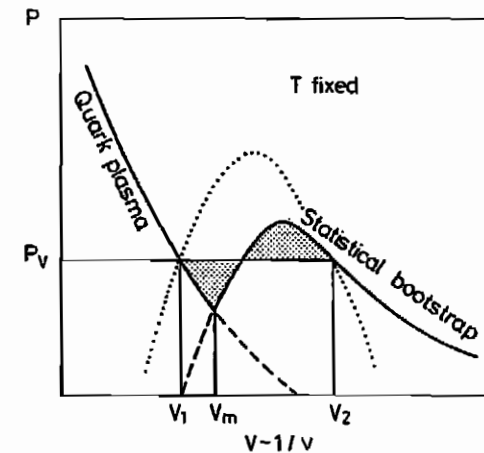
Figure 1b : P - V diagram (qualitative) of the phase transition (hadron gas to quark-gluon plasma) along the broken line T = \text{const.} of Fig. 1a. The coexistence region is found from the usual Maxwell construction (the shaded areas are equal).
