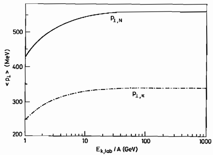
Figure 5 : Mean transverse momenta of nucleons and pions found by integrating along the "cooling curves".
