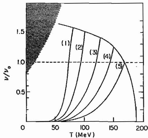
Figure 2b : The critical curve of hadron matter (bootstrap) together with some "cooling curves" (same energies as in Fig. 2a) in the variables T and v/v_0 = (\text{baryon number density})/(\text{normal nuclear baryon number density}) . In the shaded region our approach may be invalid.
