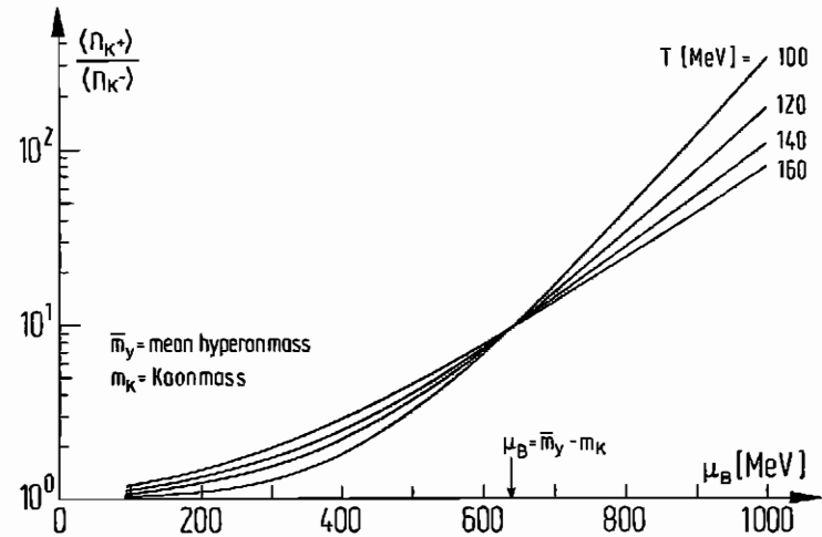
Fig. 3: The ratio \langle n_{K^+} \rangle / \langle n_{K^-} \rangle = \gamma^{-2} as function of the baryo-chemical potential for several temperatures.
