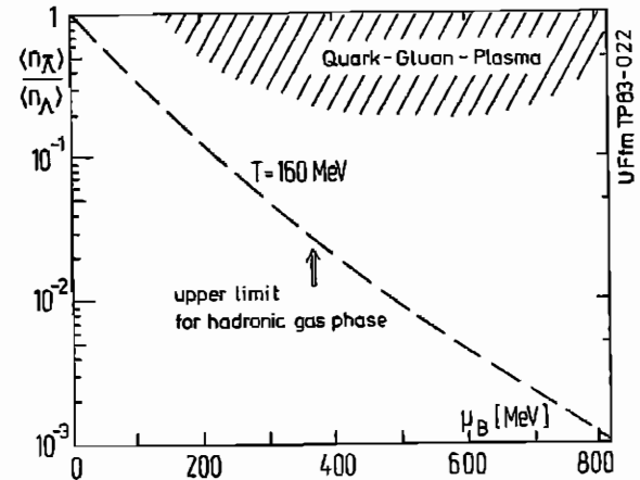
Fig. 4: Relative abundance of antilambdas: the actual yield from the hadronic gas limit may be still 10-100 times smaller than the statistical value shown.
