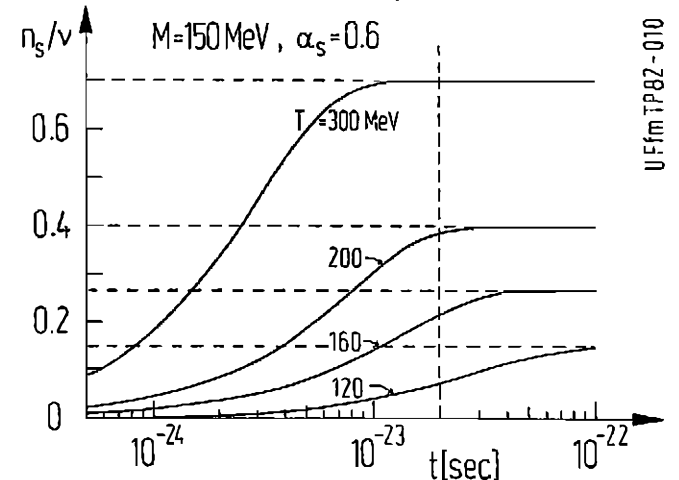
Fig. 6: Time evolution of the relative strange quark to baryon number abundance in the plasma for various temperatures T . M = 150 MeV, \alpha_s = 0.6 .
