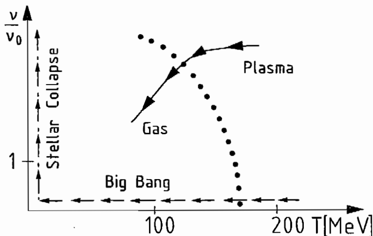
Fig. 2: Paths taken in the \nu - T plane by different physical events.
