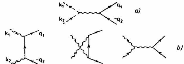
Fig. 5: Lowest order QCD diagrams for ss production: a) qq + s\bar{s} ; b) gg + s\bar{s} .
