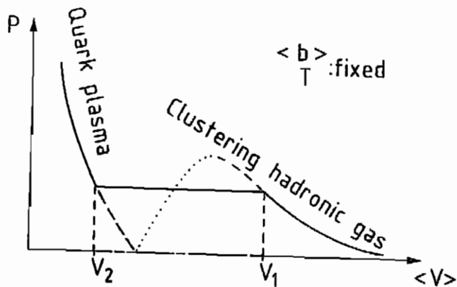
Fig. 1: p - V diagram for the gas-plasma first order transition, with the dots indicating a model-dependent, unstable domain between overheated and undercooled phases.
