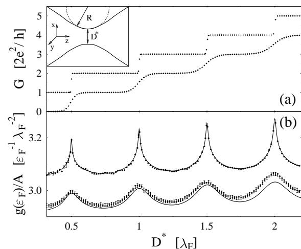
FIG. 1. Inset: Schematic diagram of a metallic nanocontact. (a) Conductance G and (b) DOS g(\varepsilon_F) for 2D nanocontacts with \alpha \approx 5 versus the contact diameter D^* . g is normalized to the area A of the region. Solid curves: semiclassical result based on Eq. (8); crosses with error bars: numerical results using the method of Ref. [10]. Lower curves in (a) and (b): R \approx \lambda_F ; upper curves (offset vertically): R \approx 170\lambda_F .
