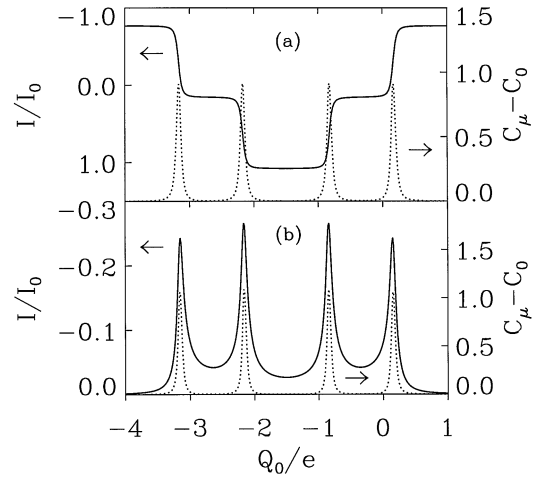
FIG. 2. Persistent current and differential capacitance as a function of the polarization charge Q_0 = C_e V for (a) the sample of Fig. 1(a) with t = 0.5 and (b) the sample of Fig. 1(b) with t_R = 0.2 and t_L = 0.3 . Each sample contains six electrons, with \Phi/\Phi_0 = 1/4 , and e^2/C = 10 . Energy is expressed in units of w , 4w being the bandwidth in the ring. The persistent current (solid curve) is expressed in units of I_0 = \max(ev_F/L) , where L is the circumference of the ring, and the capacitance (dotted curve) is expressed in units of (C_e/C)^2 e^2/w . Each peak in C_\mu corresponds to the transfer of one electron from the dot to the ring.
