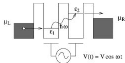
FIG. 1. Schematic diagram of the double-quantum-dot electron pump.
