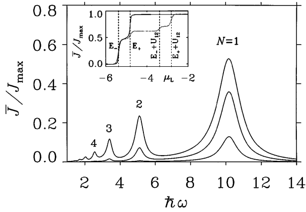
FIG. 3. Time-averaged current \bar{J} (in units of J_{\max} = e\Gamma/2\hbar ) through a double quantum dot with \epsilon_1 = -5 , \epsilon_2 = 5 , \Gamma = 0.5 , and ac amplitude V = 2, 4, 6 (increasing \bar{J} ). Energies are given in units of w , the tunneling matrix element between the dots. With \mu_L = \mu_R = 0 , the system functions as an electron pump due to coherent N -photon-assisted tunneling, with resonances at \omega_N = (\Delta\epsilon^2 + 4w^2)^{1/2}/N\hbar . Inset: time-averaged current at the one-photon resonance \omega = \omega_1 vs dc bias \mu_L , with V = 6 . Solid curve: U_{12} = 0 , \Gamma = 0.05 , k_B T = 0 ; dotted curve: U_{12} = 2 , k_B T = 0.05 \gg \Gamma . The jumps, of width \max(k_B T, \Gamma) , of \bar{J} at E_{\pm} and E_{\pm} + U_{12} allow one to resolve the Rabi splitting |E_+ - E_-| \approx 2wJ_1(V/\hbar\omega) = 0.563 and the interdot interaction U_{12} .
