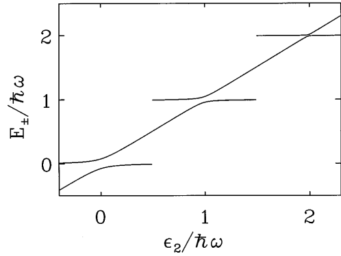
FIG. 2. Exact quasienergies of two coupled quantum dots vs detuning \epsilon_2 . Here \epsilon_1 = V \cos\omega t , with V = \hbar\omega = 10w . Note that the quasienergies are defined mod( \hbar\omega ). The electronic states on the dots hybridize and split by \approx 2wJ_N(V/\hbar\omega) , becoming delocalized, when \epsilon_2 crosses the N th sideband of \epsilon_1 .
